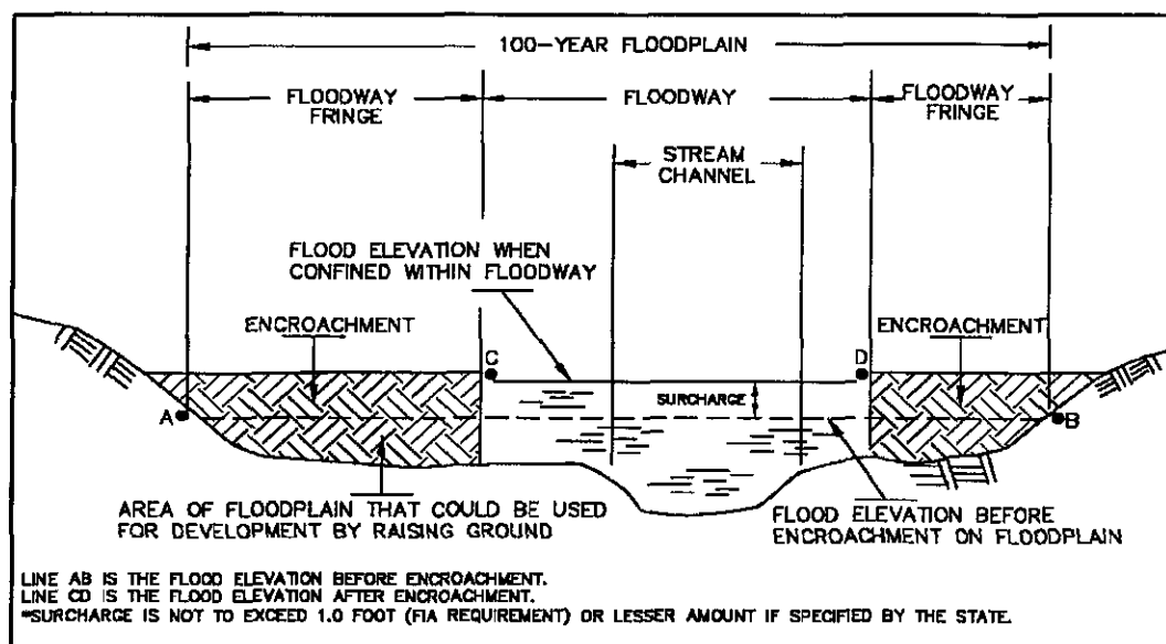
Figure 3: Floodway Schematic
